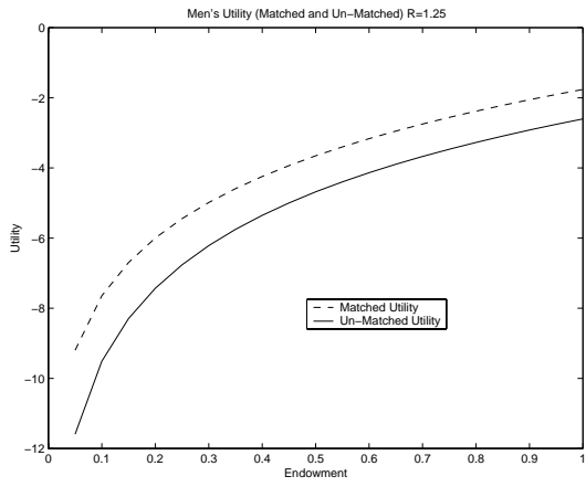
Figure 5: Utility and Surplus, R=1.25
